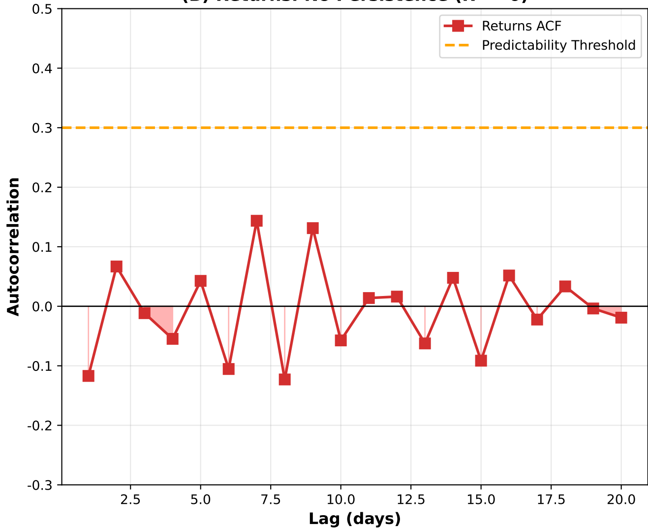
(B) Returns: No Persistence ( R^2 \approx 0 )
