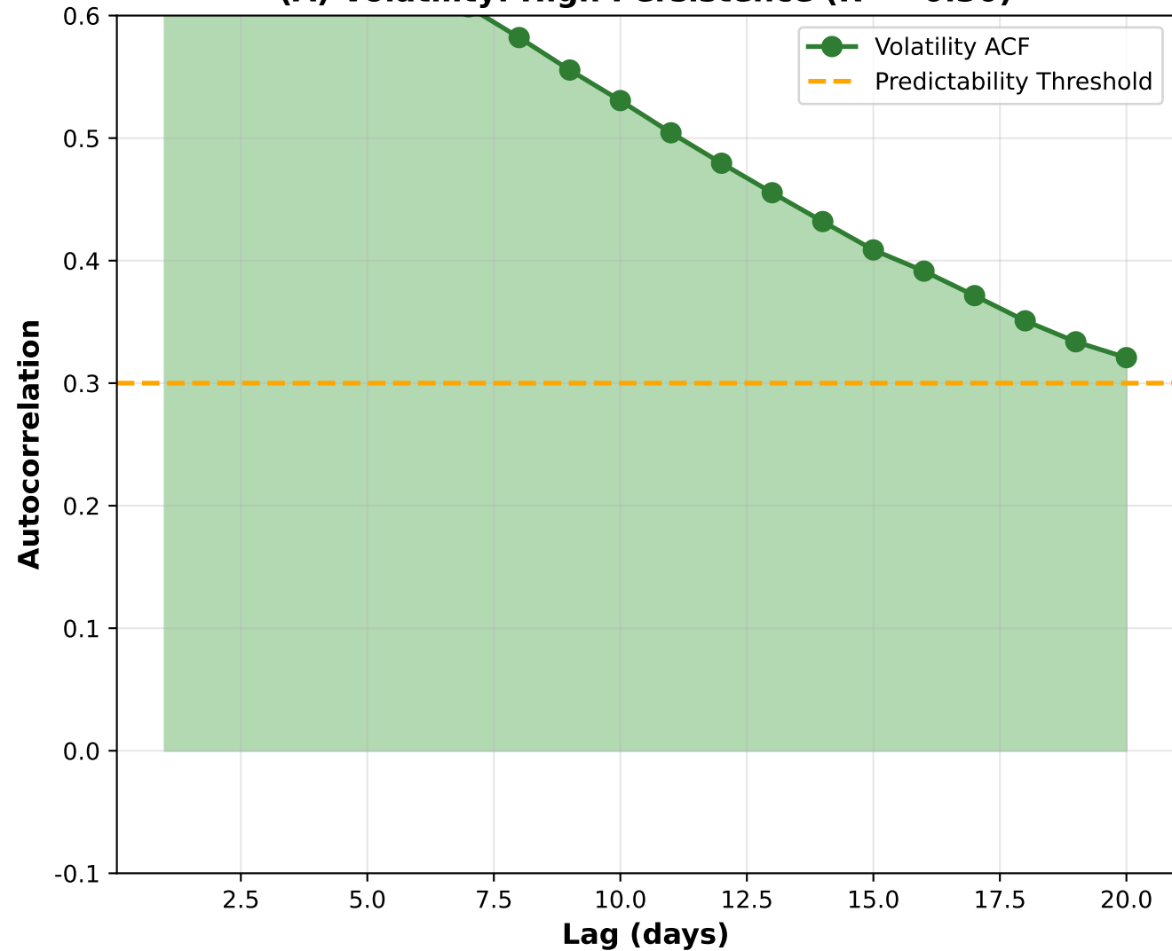
(A) Volatility: High Persistence ( R^2 = 0.30 )
