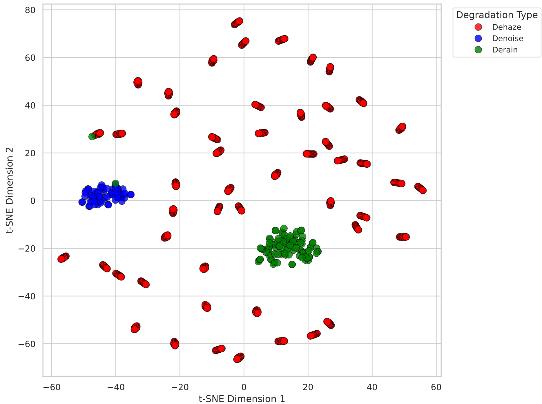
Latent Layer Feature Embedding (t-SNE)
