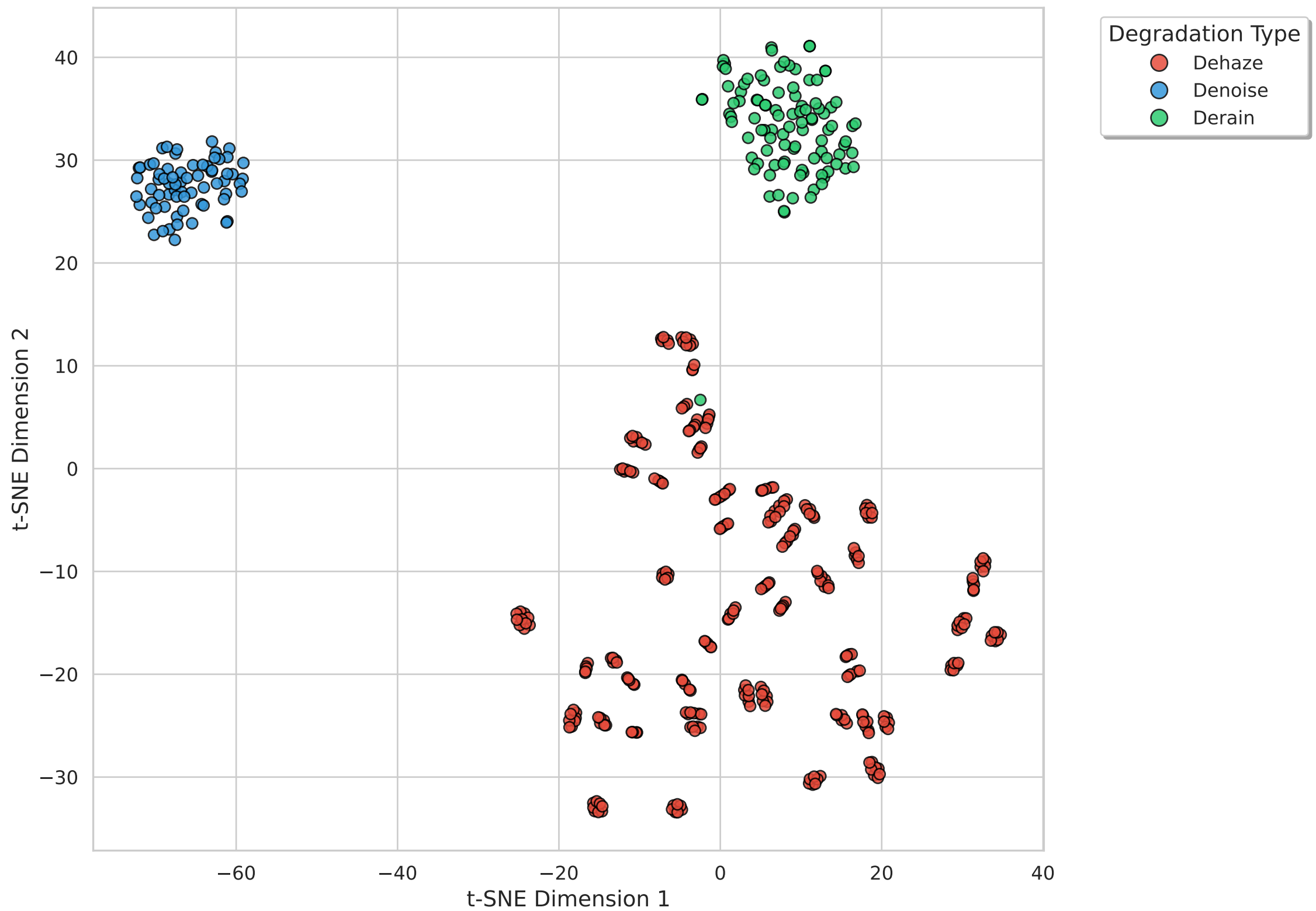
Latent Layer Feature Embedding (t-SNE) - Balanced Samples
