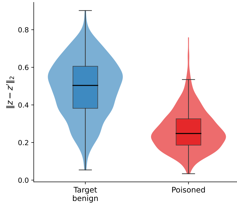
(c) Representation response
