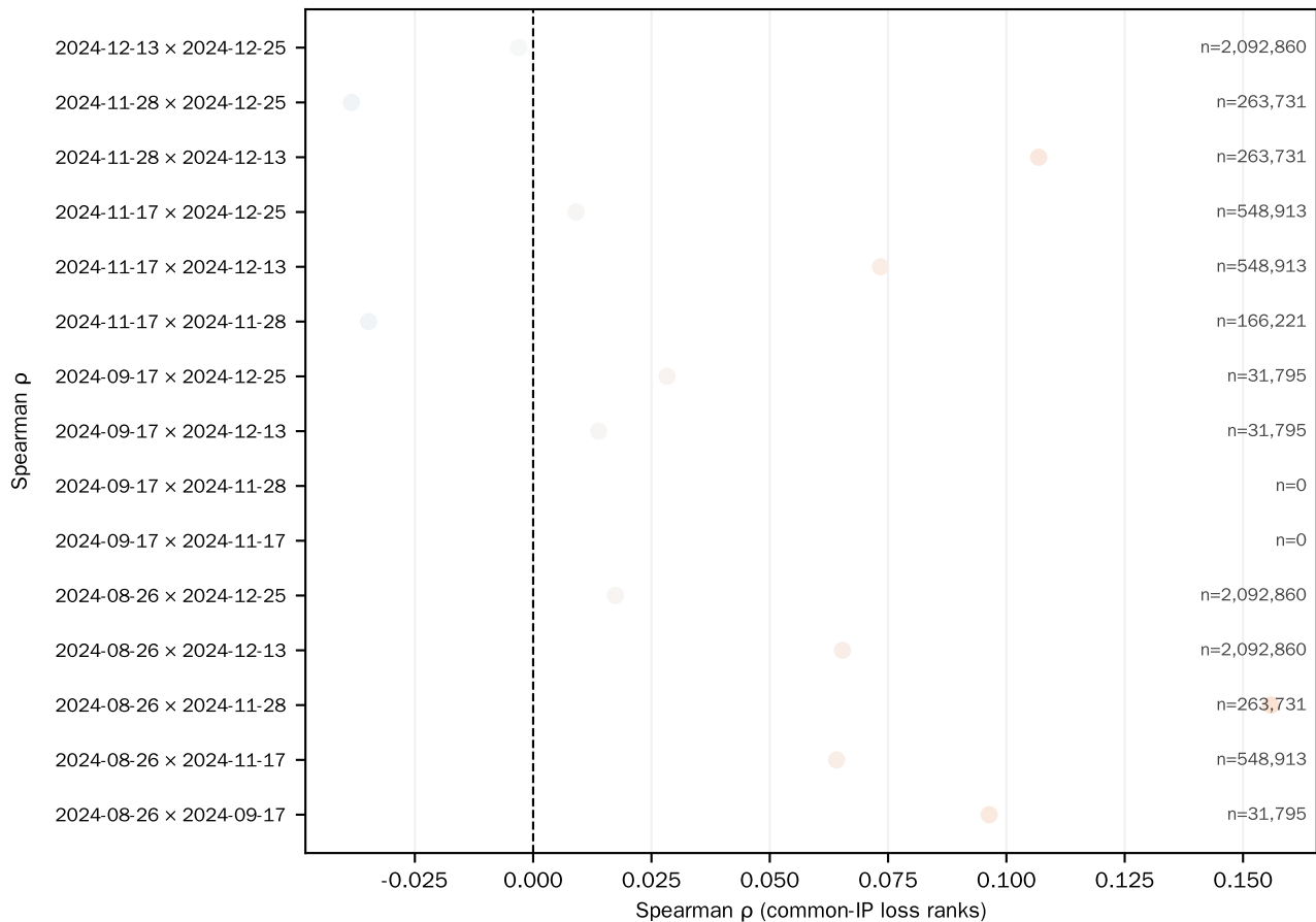
(b) Event-pair dot plot
