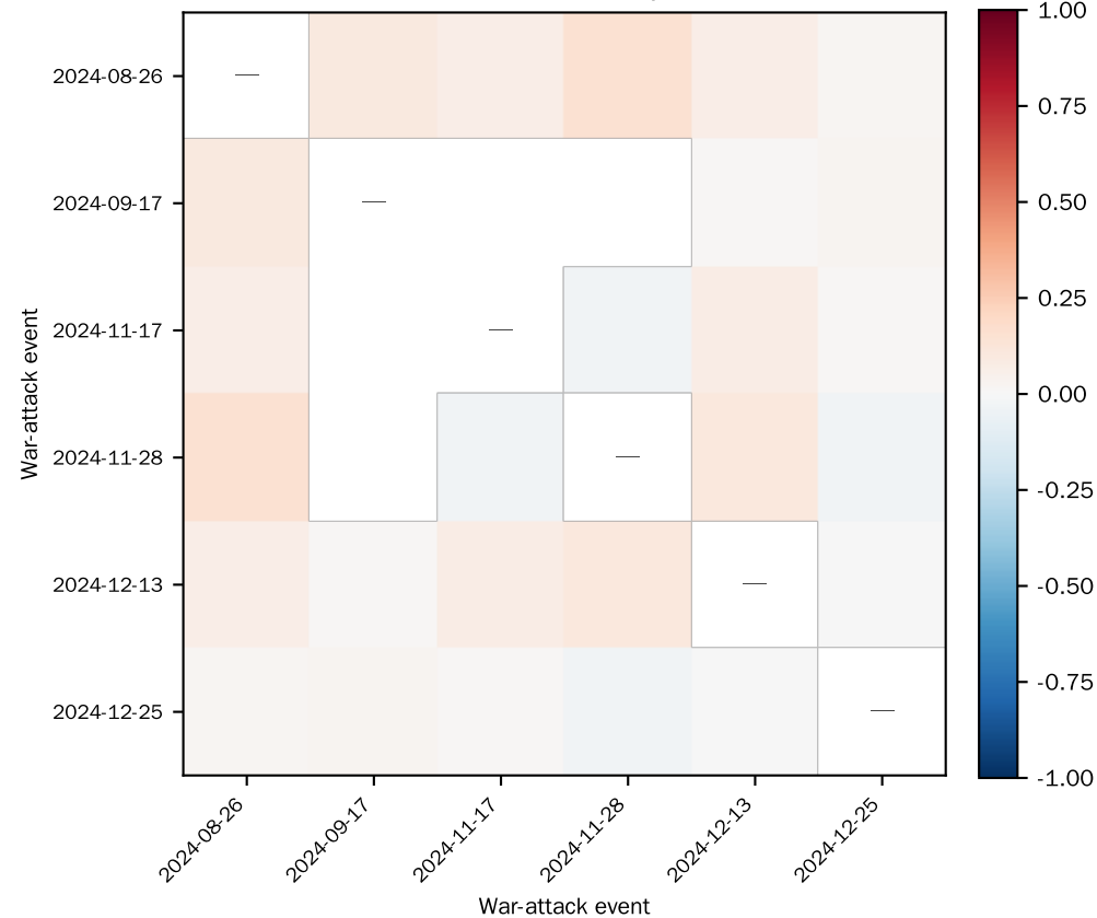
(a) Event-pair Spearman \rho heatmap
