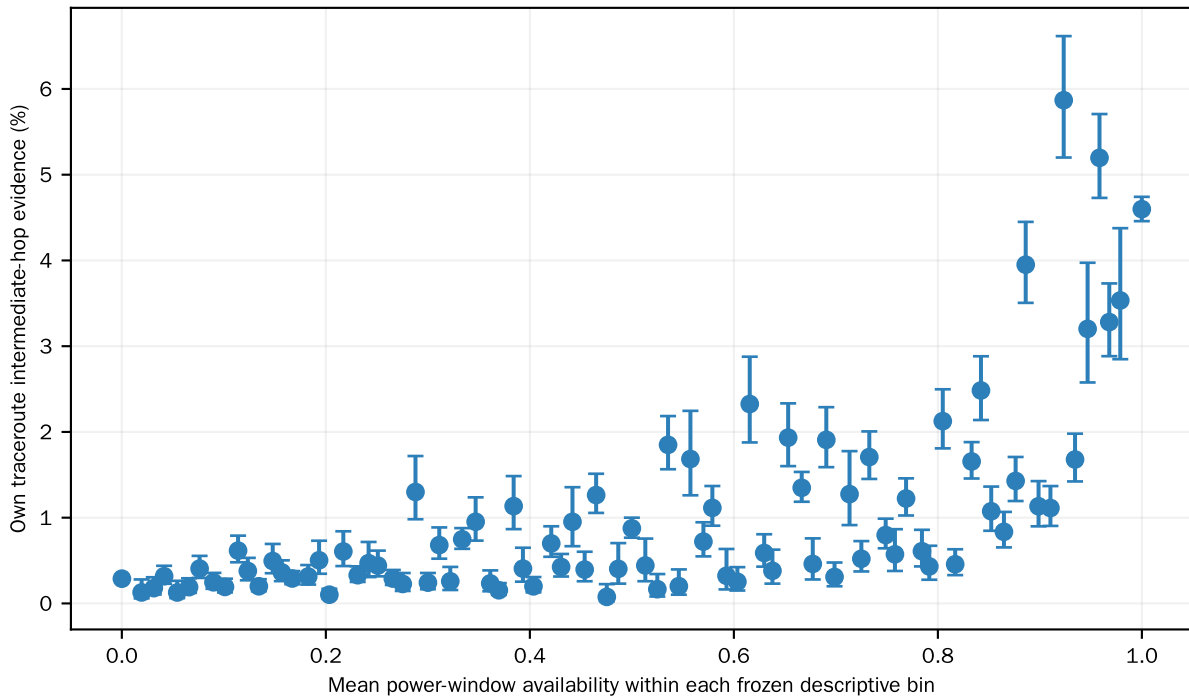
Own Traceroute Intermediate-Hop Evidence and Power-Window Availability
