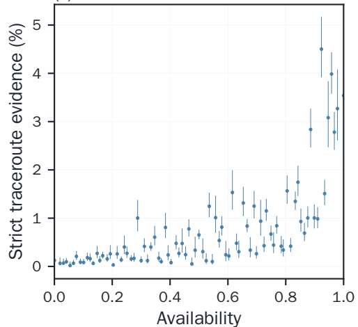
(c) Strict traceroute evidence
