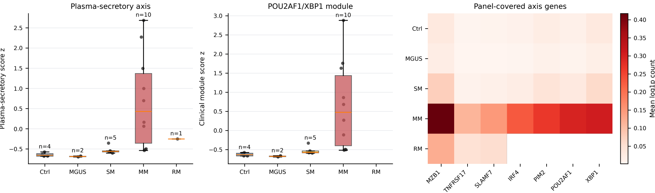
Fig. 4 | GSE299193 Xenium spatial reproducibility of the plasma-secretory program
