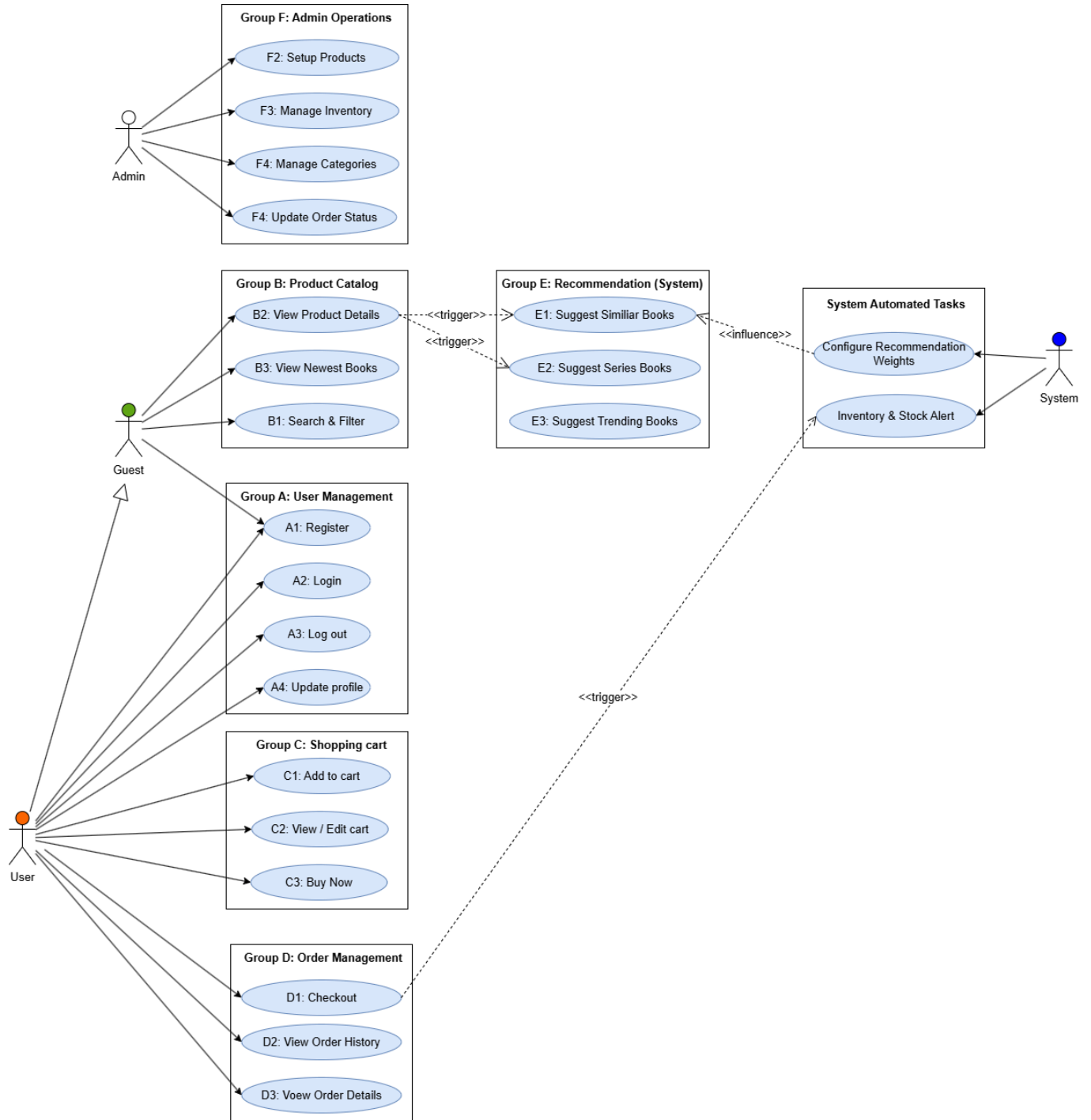
Figure 1.4 Overview of the system's actors and use cases.
