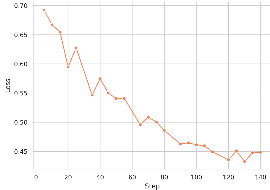
Training Loss
