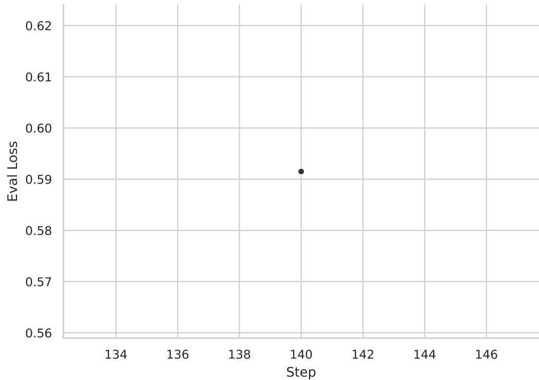
Validation Loss
