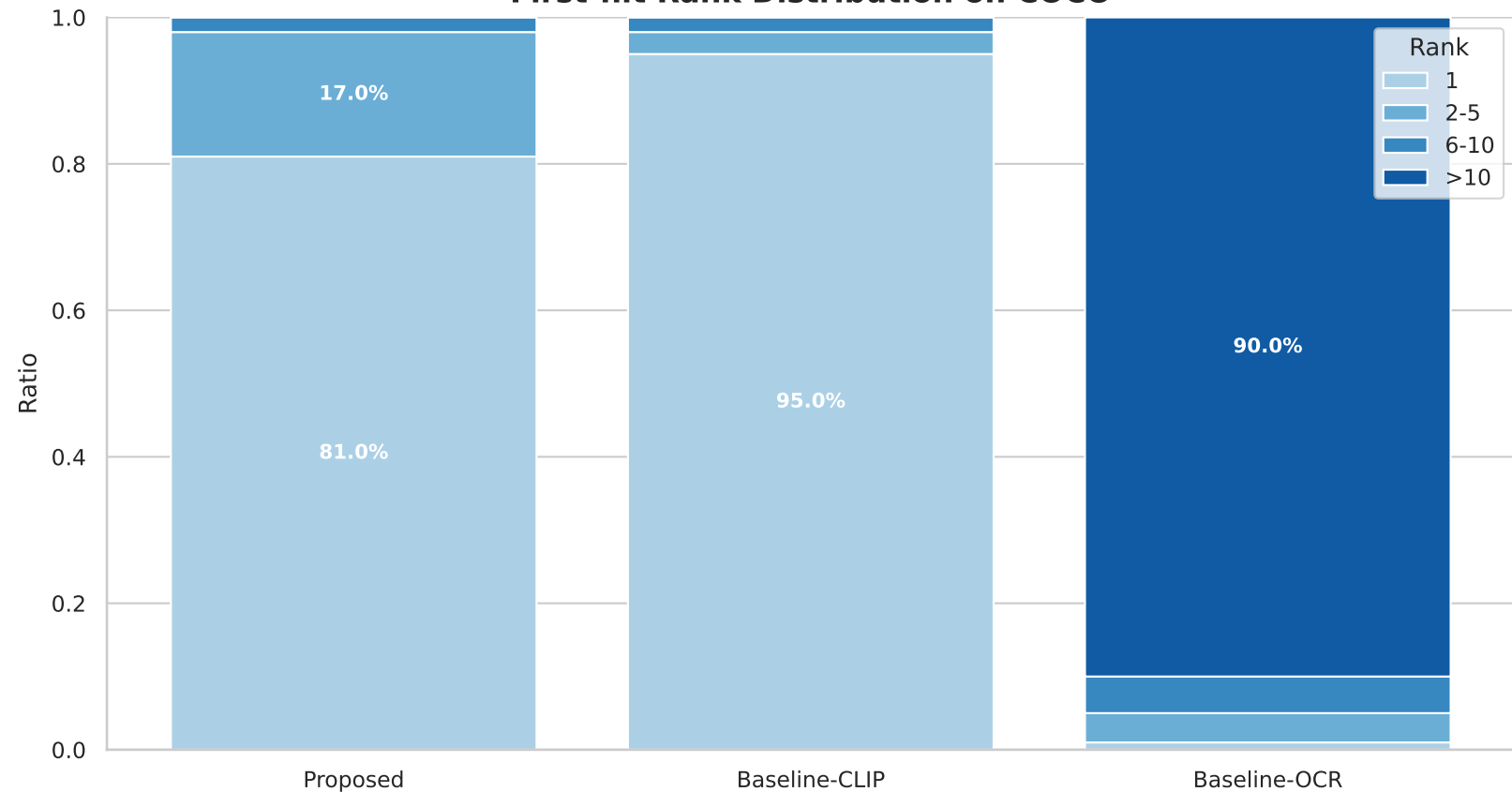
First-hit Rank Distribution on COCO
