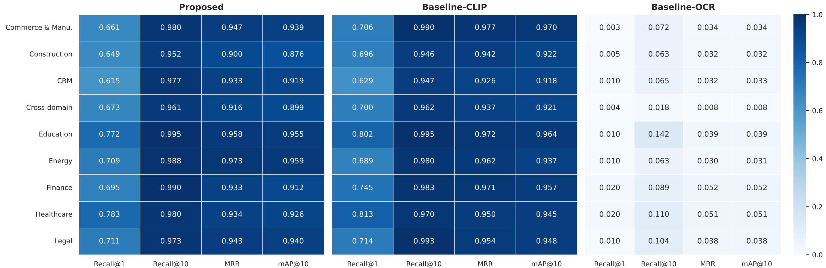
Domain-level Metric Heatmaps
