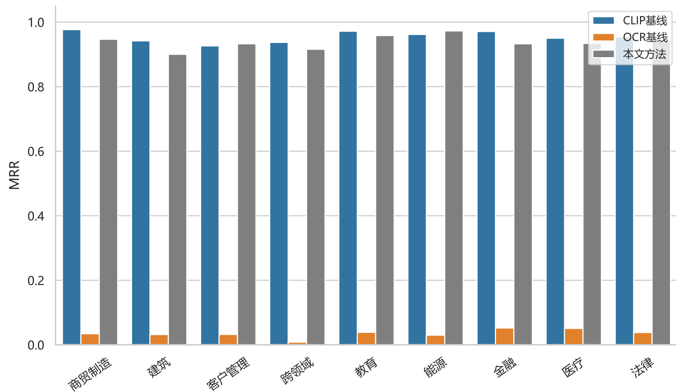
MRR
