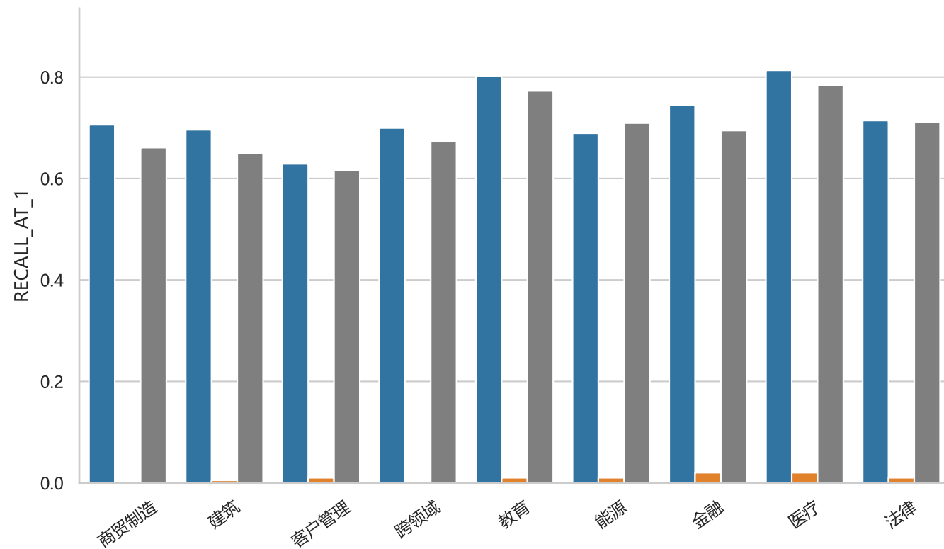
Recall@1
