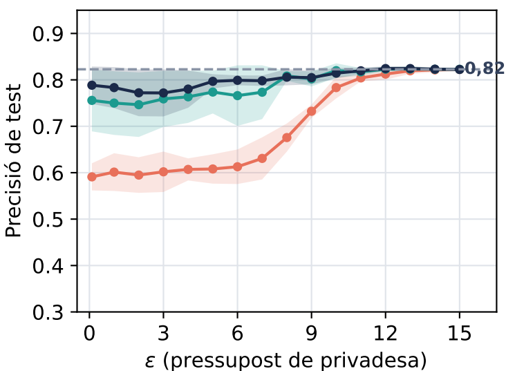
Pubmed
