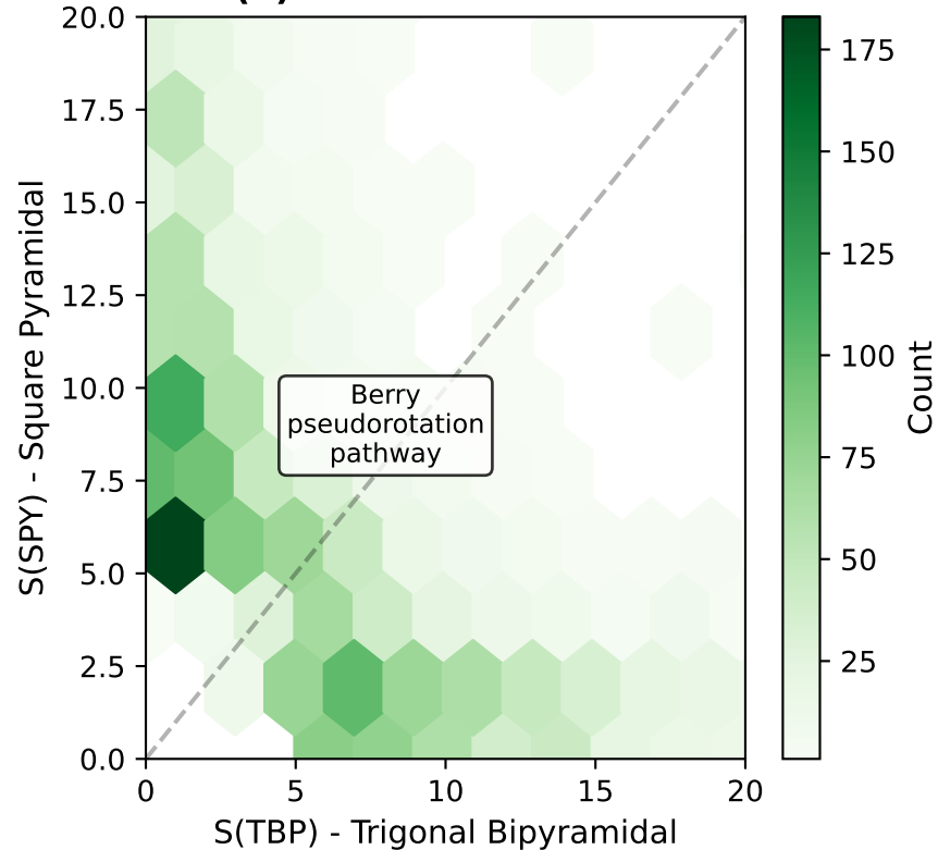
(b) CN=5: TBP vs SPY
