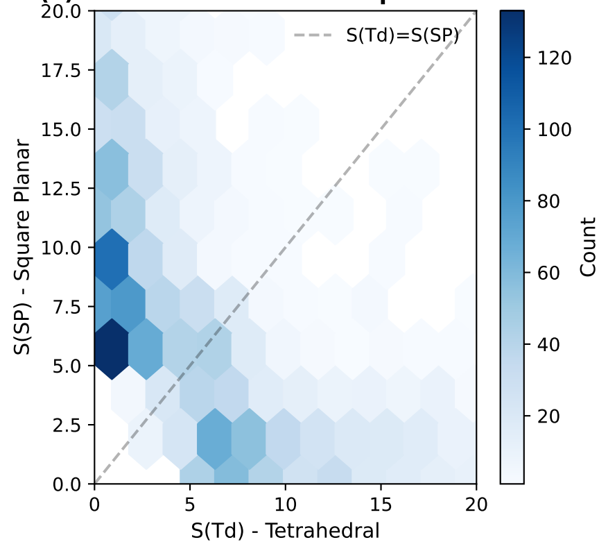
(a) CN=4: Tetrahedral vs Square Planar
