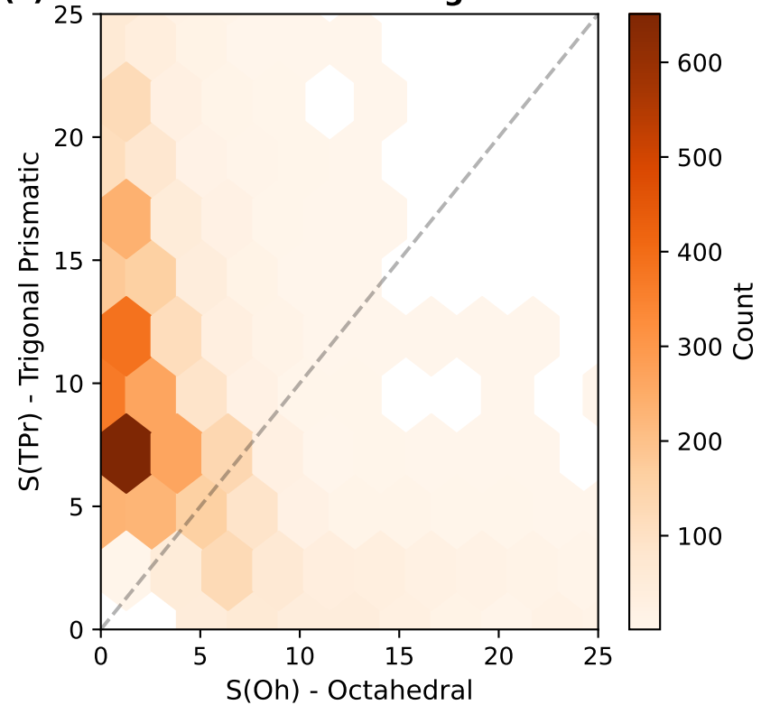
(c) CN=6: Octahedral vs Trigonal Prismatic
