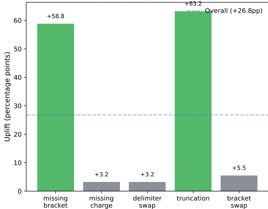
(b) Repair Uplift by Corruption Type
