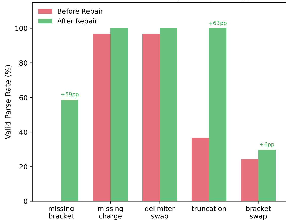
(a) Repair Performance by Corruption Type
