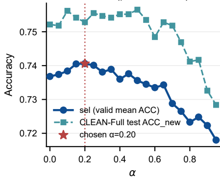
Math1 (peak \alpha=0.20 )
