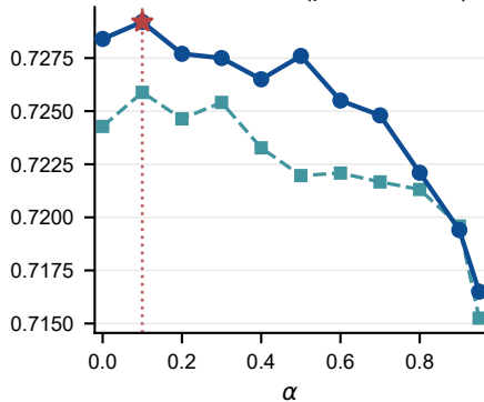
ASSIST a0910 (peak \alpha=0.10 )
