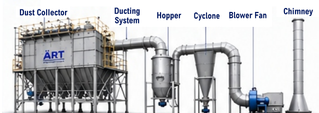
COMPLETE INTEGRATED DUST COLLECTION SYSTEM
