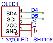
1.3寸OLED : SH1106
