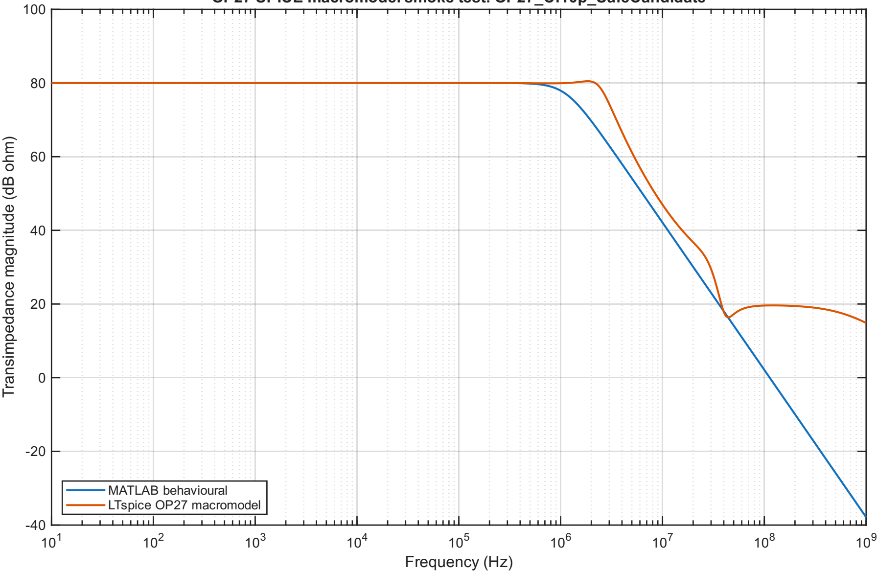
OP27 SPICE macromodel smoke test: OP27_Cf10p_SafeCandidate
