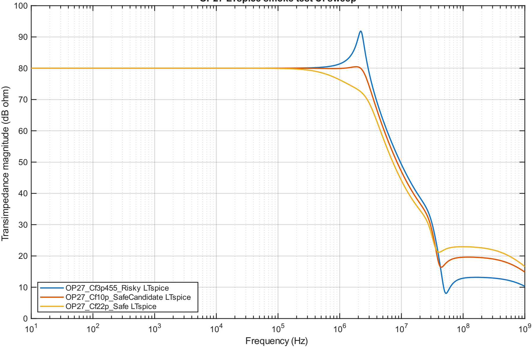
OP27 LTspice smoke test Cf sweep
