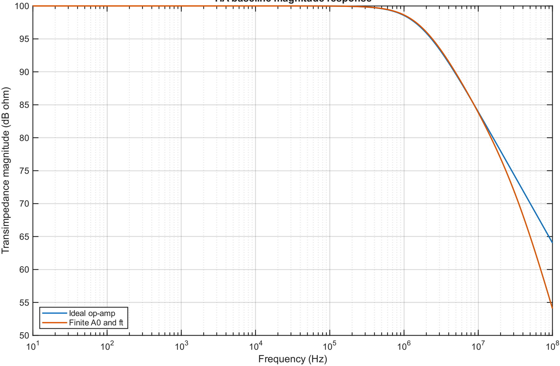
TIA baseline magnitude response
