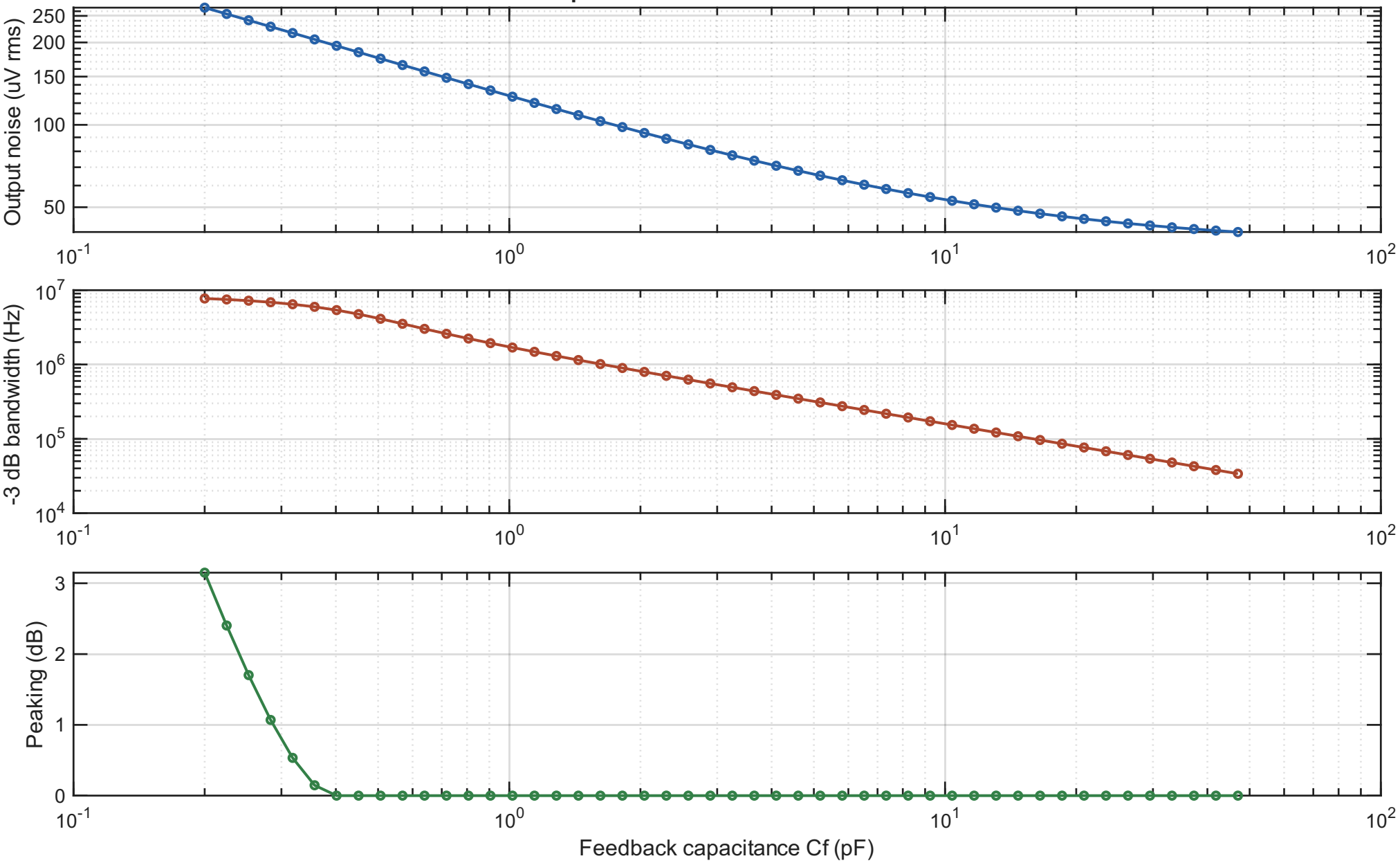
First-pass TIA noise-bandwidth trade-off
