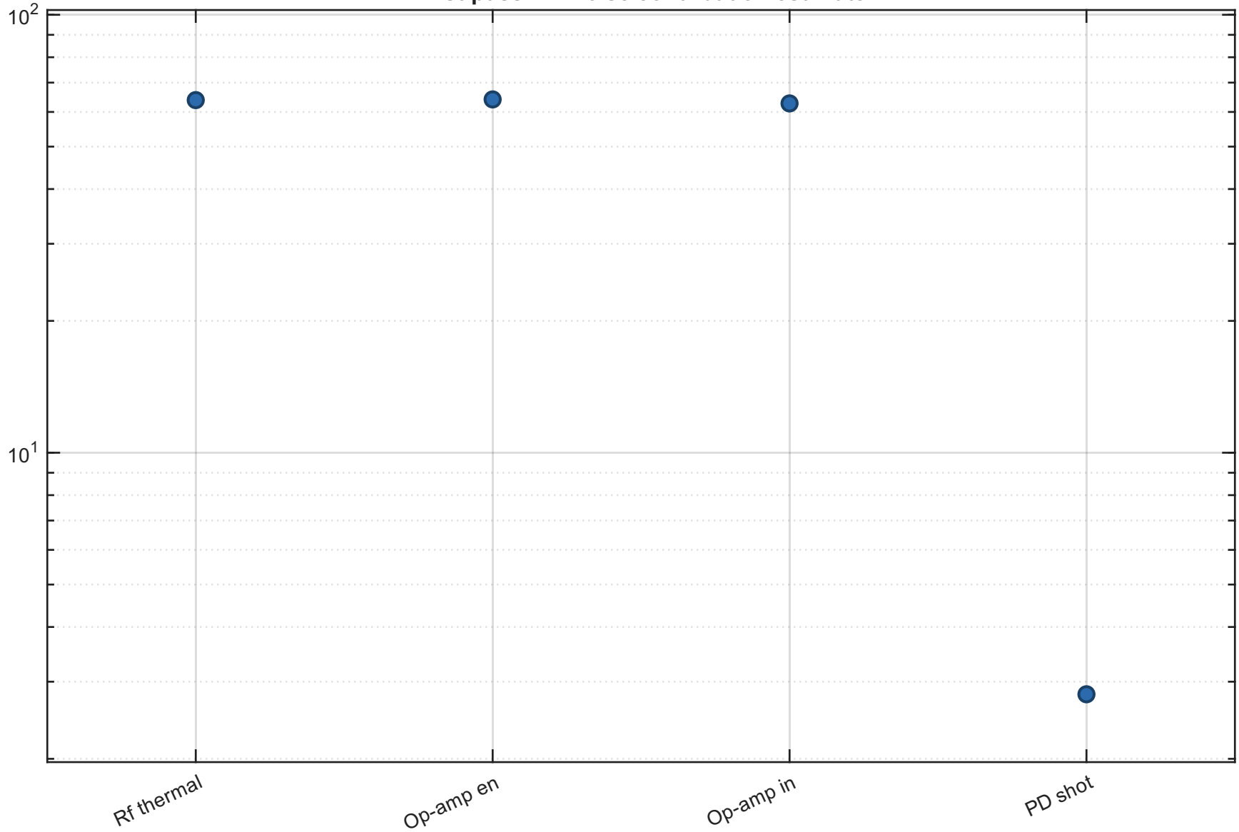
First-pass TIA noise contribution estimate
