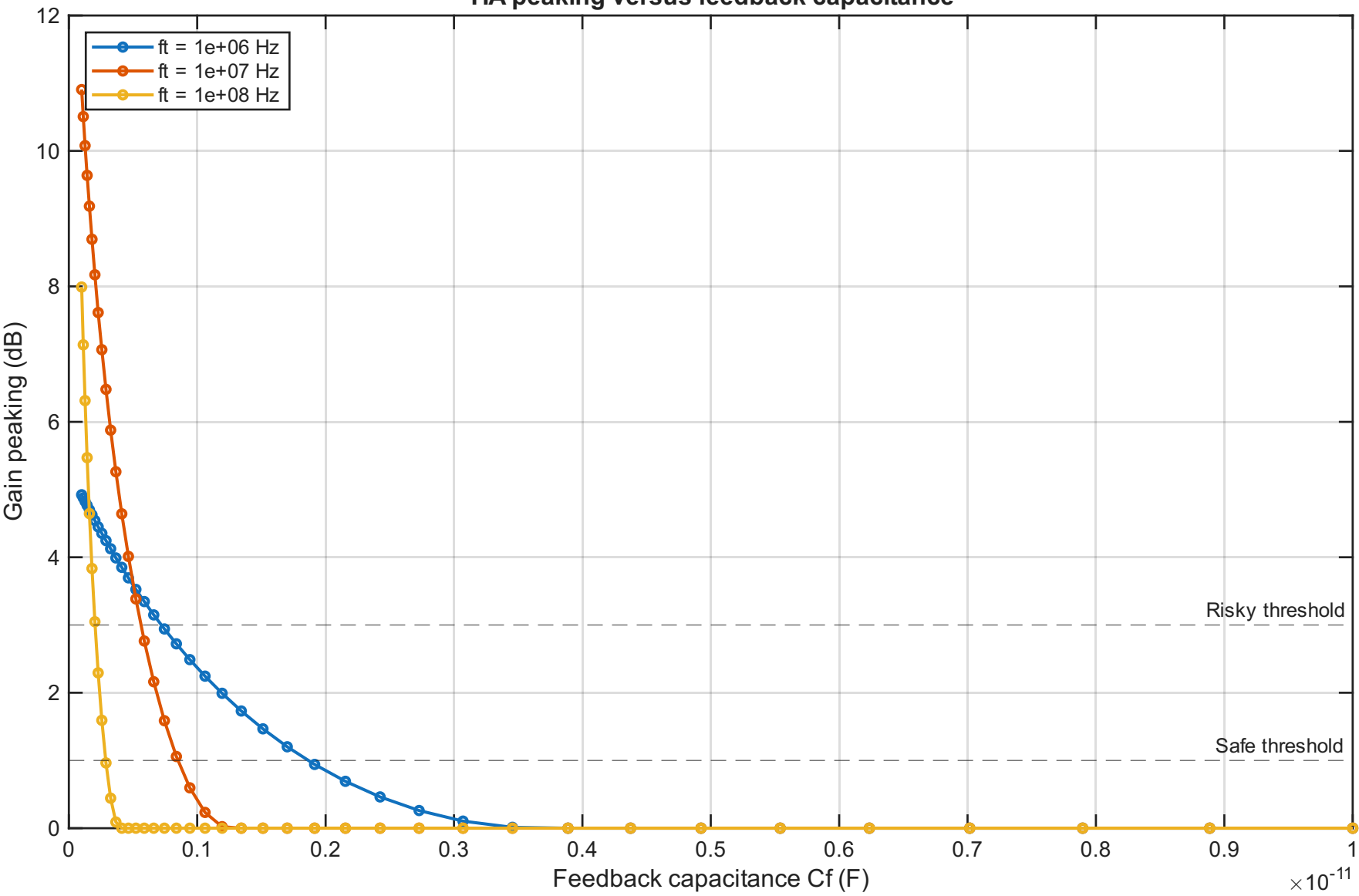
TIA peaking versus feedback capacitance
