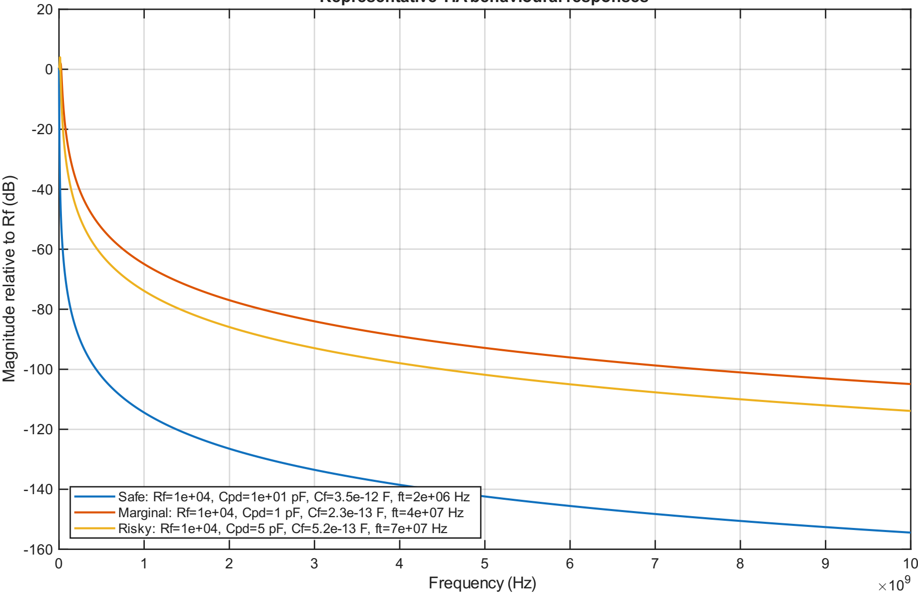
Representative TIA behavioural responses
