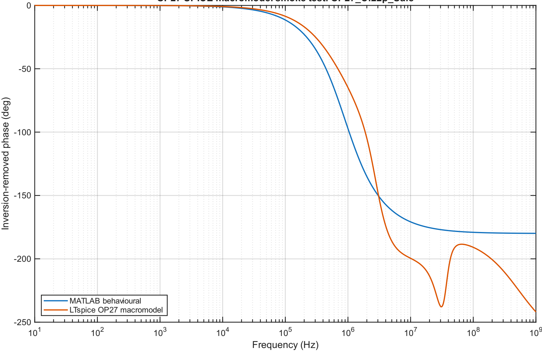
OP27 SPICE macromodel smoke test: OP27_Cf22p_Safe
