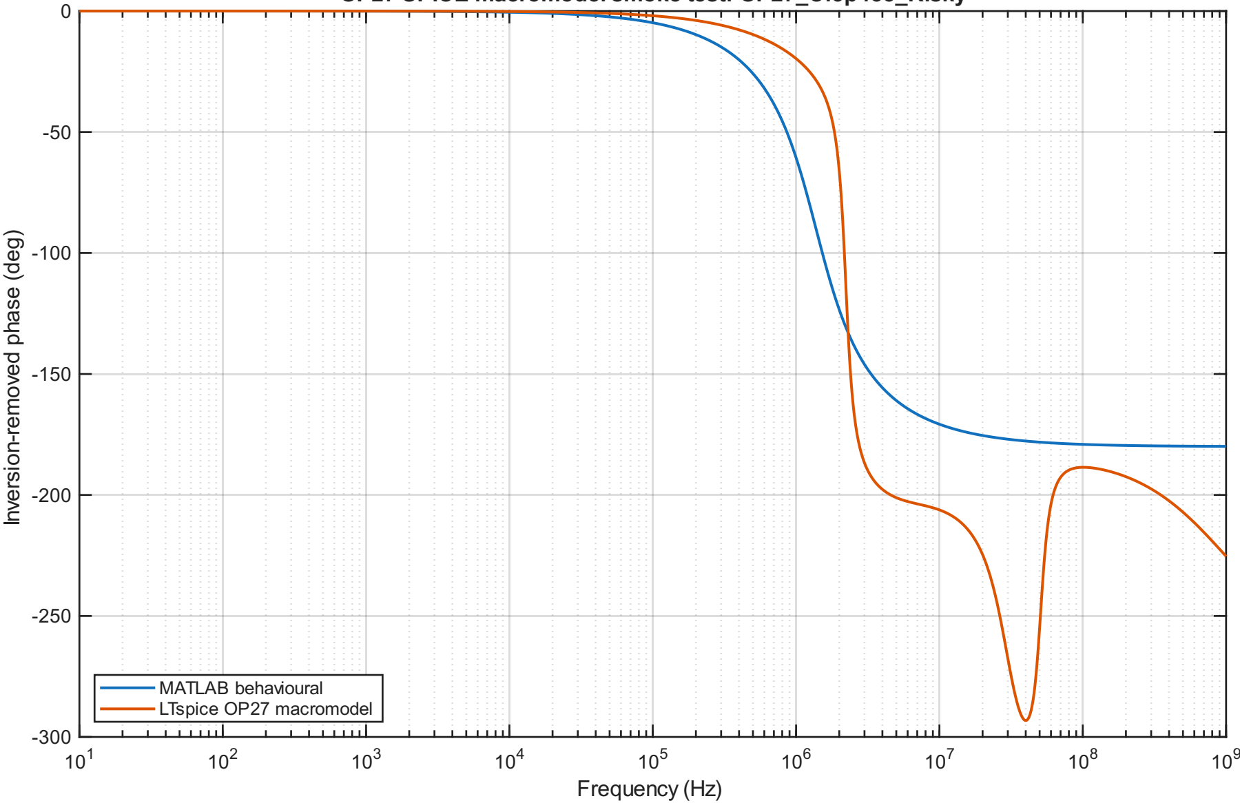
OP27 SPICE macromodel smoke test: OP27_Cf3p455_Risky
