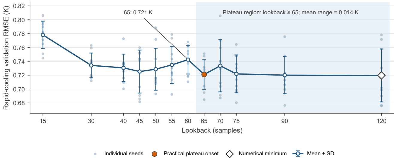
Lookback sensitivity for the 15-step Thv forecast (n = 10 seeds)
