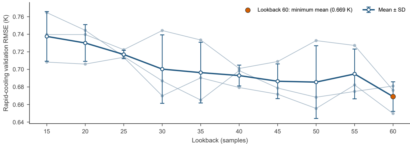
Lookback sensitivity for the 15-step Thv forecast
