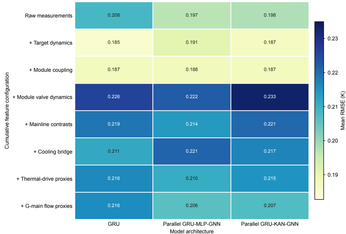
Validation RMSE across models and cumulative features
