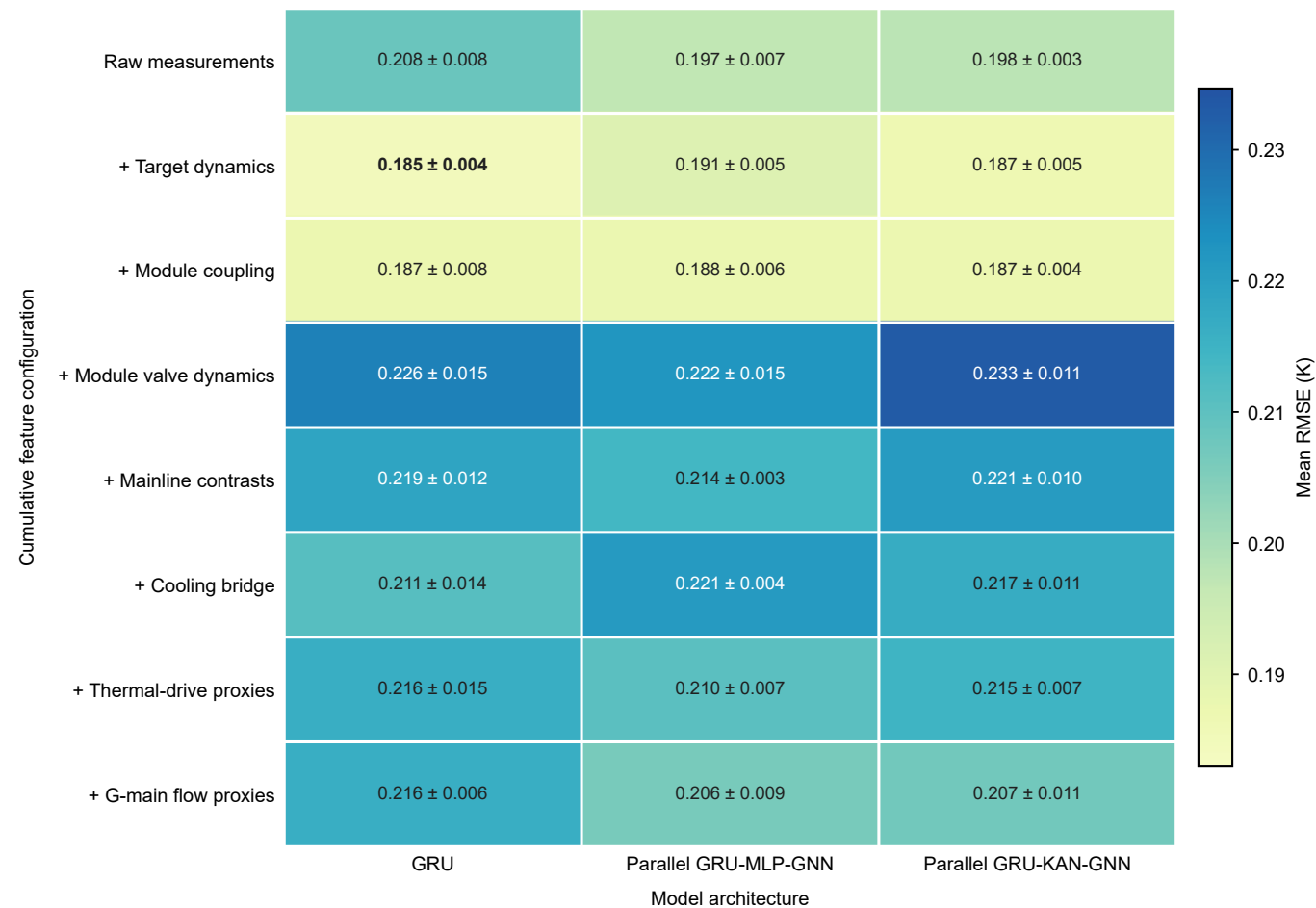
Validation RMSE across architectures and cumulative features
