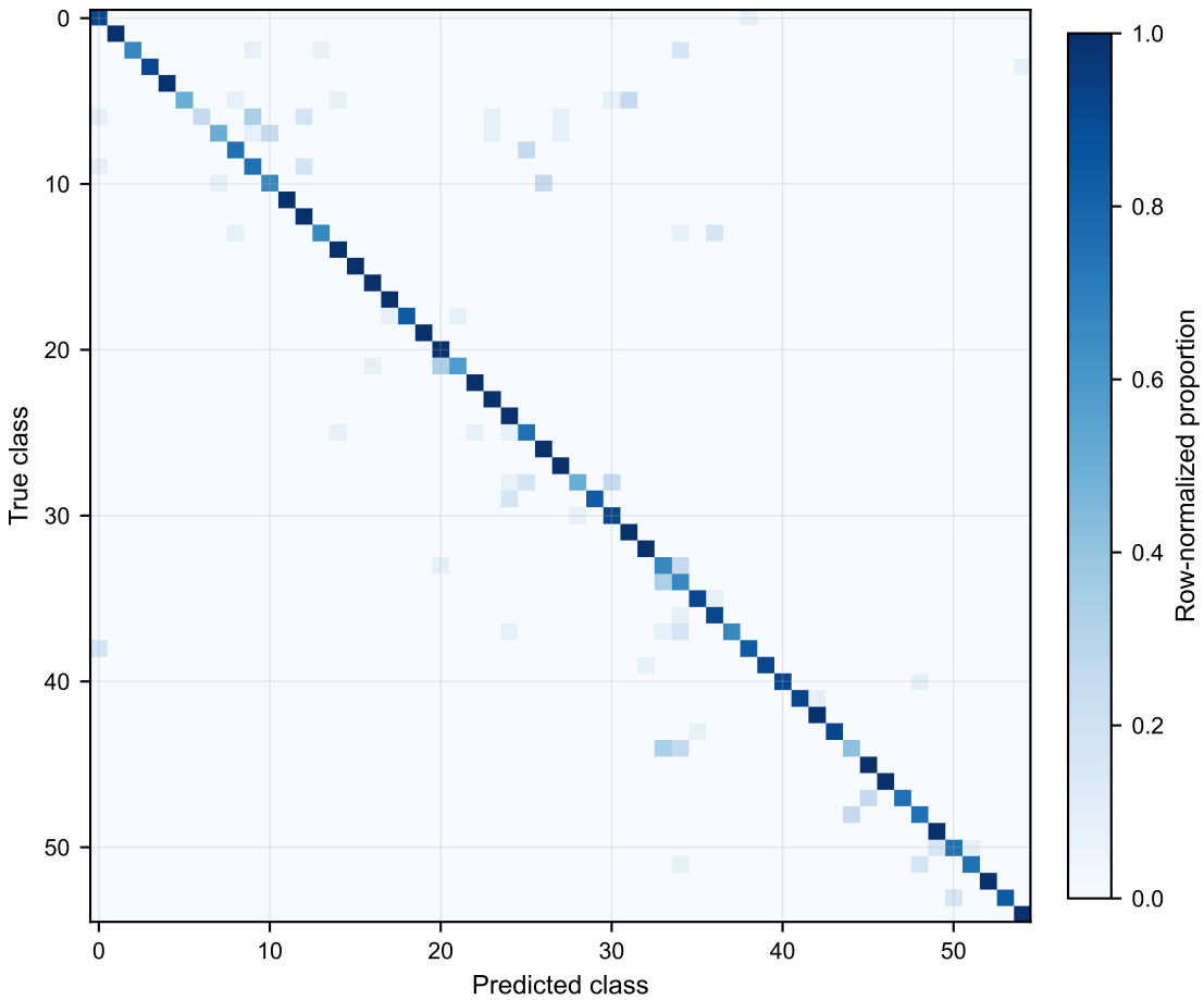
XRF55 without Hampel
