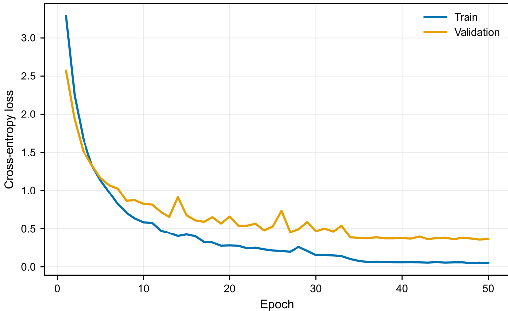
XRF55 without Hampel, model seed=42
