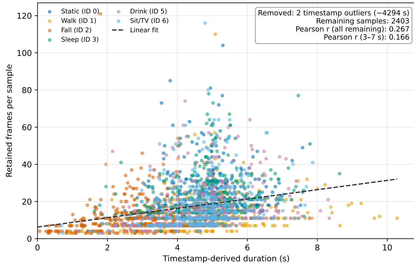
ElderAL retained frames vs. timestamp-derived duration (two timestamp outliers removed)
