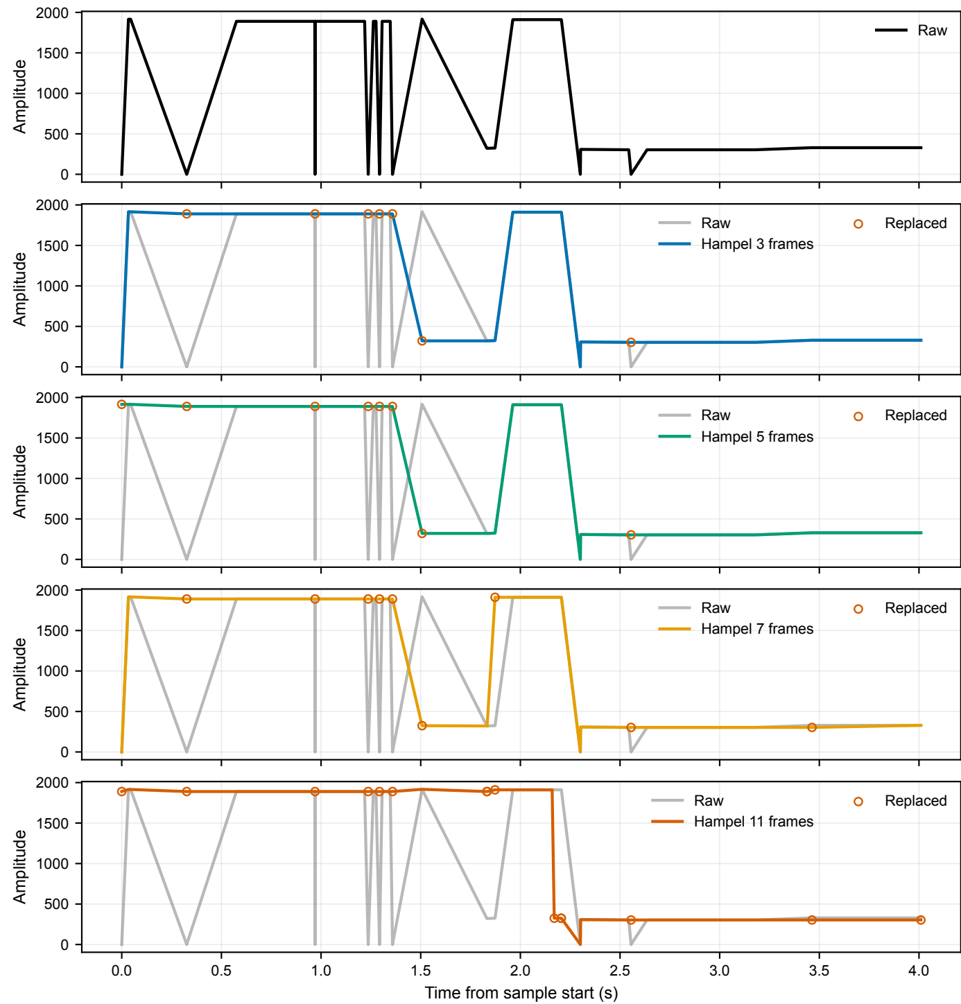
Representative ElderAL channel: 20250813=204917_mimo5s_part0.csv, subcarrier=257, link=2
