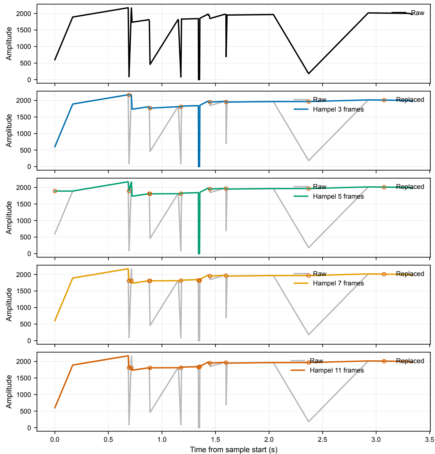
Representative ElderAL channel: 20250813=230850_mimo5s_part0.csv, subcarrier=193, link=2
