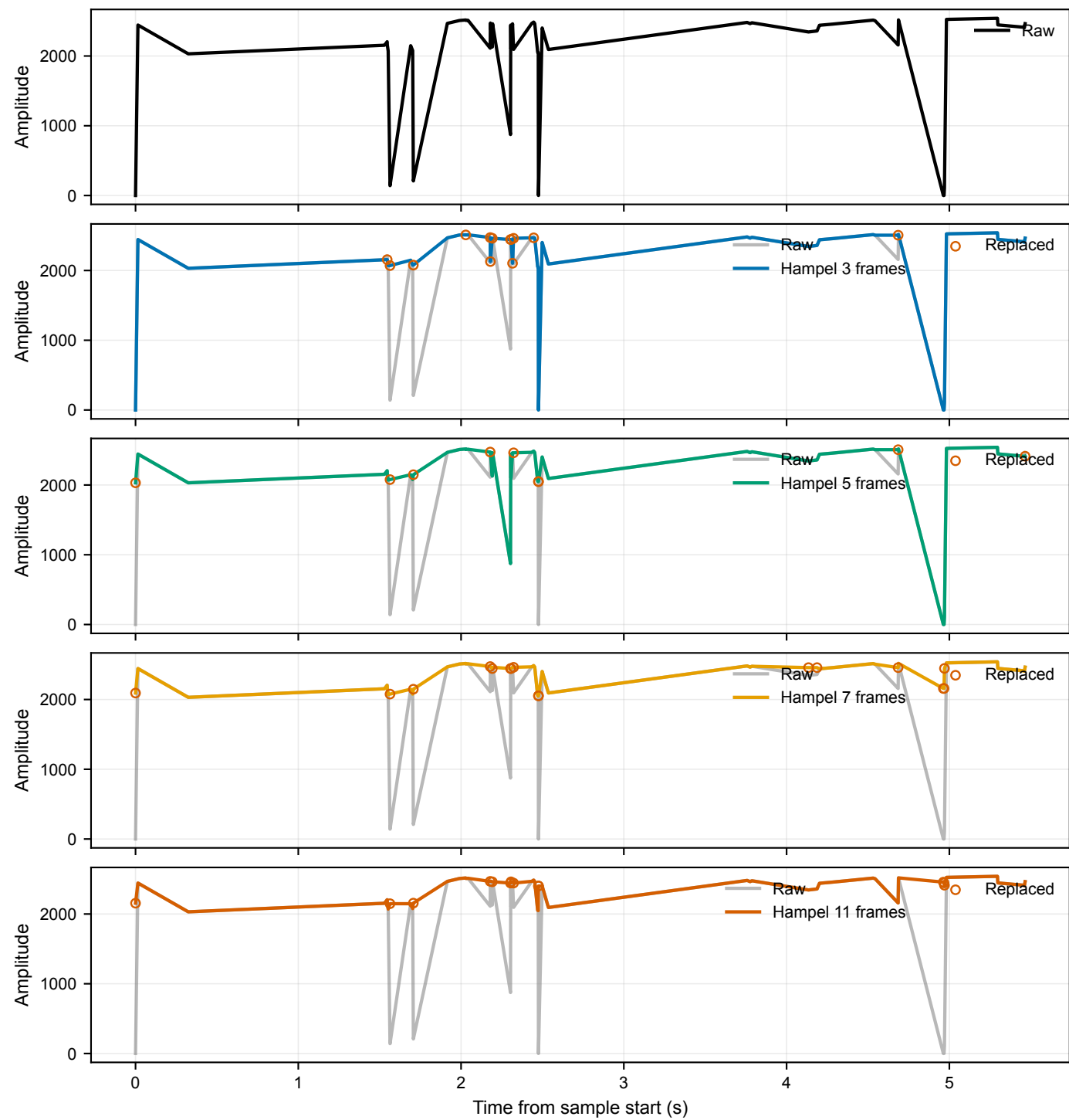
Representative ElderAL channel: 20250813=171349_mimo5s_part0.csv, subcarrier=139, link=2
