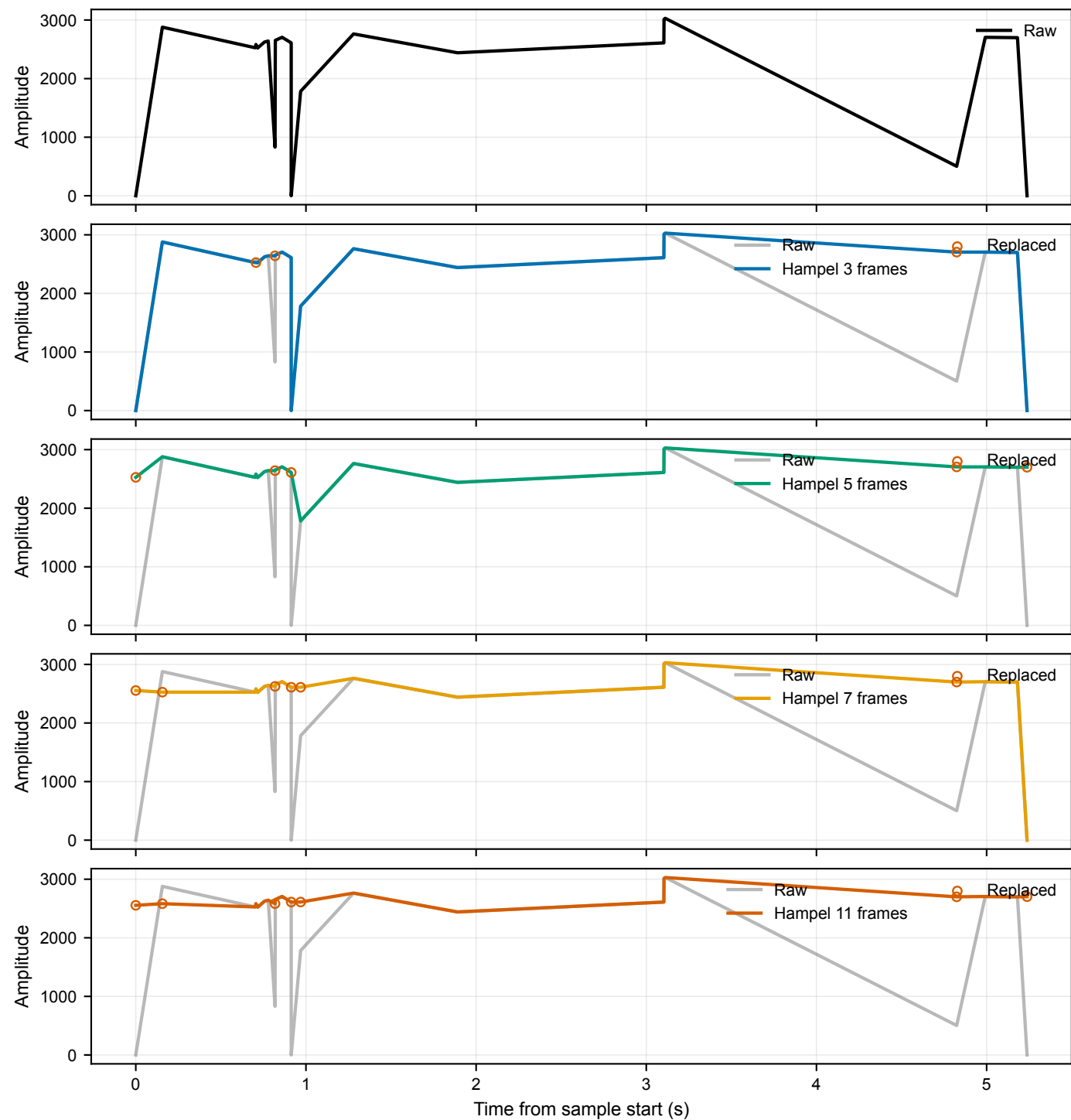
Representative ElderAL channel: 20250813=122048_mimo5s_part0.csv, subcarrier=322, link=2
