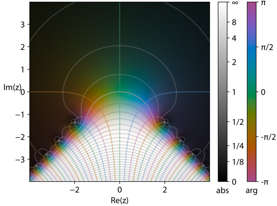
Figure 2.1: Values of the Faddeeva function inside the complex plane (Wikipedia's picture).
