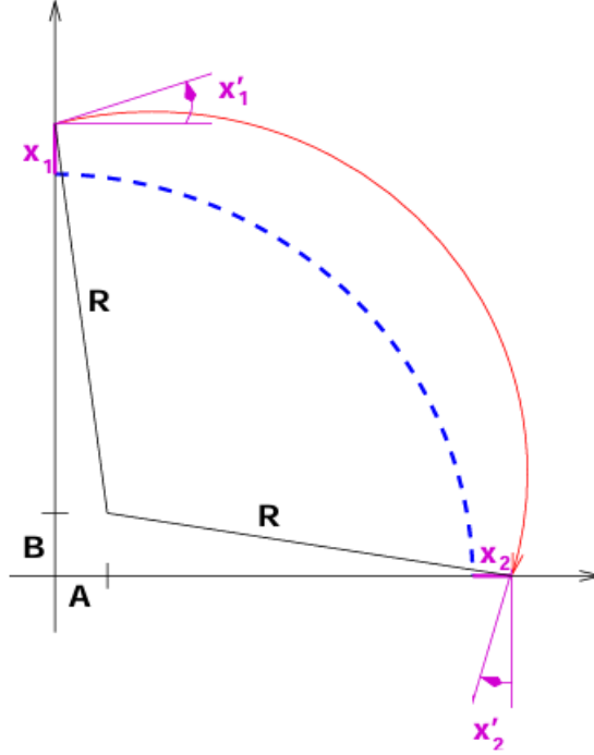
Figure 1.1: Geometry of the particle trajectory in a 90^\circ bending magnet. Figure taken from [15]
