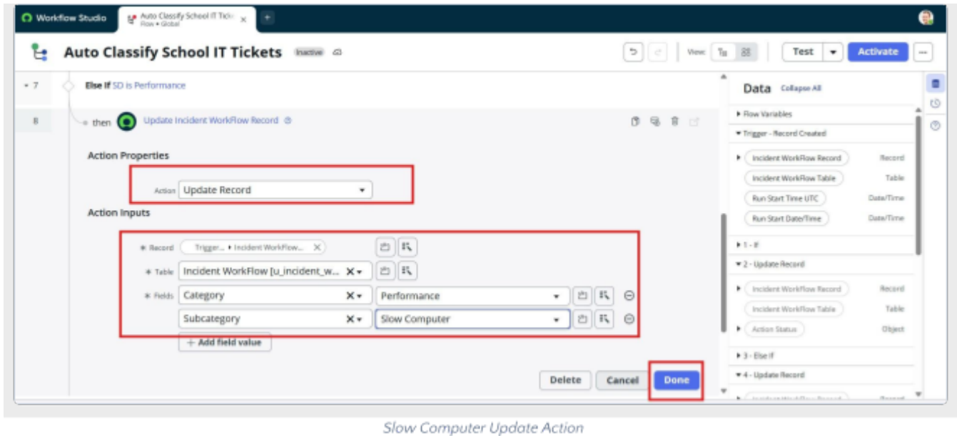
Figure 6.10: Performance / Slow computer classification logic.
