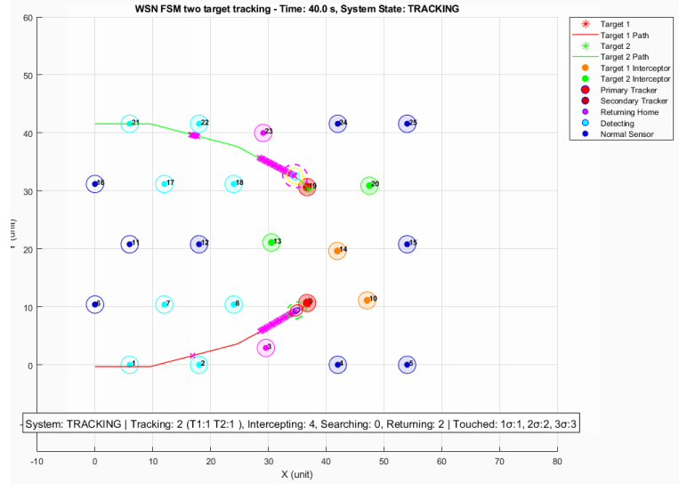
Figure 4: Proposed affected-target expansion at t = 40.0s .
