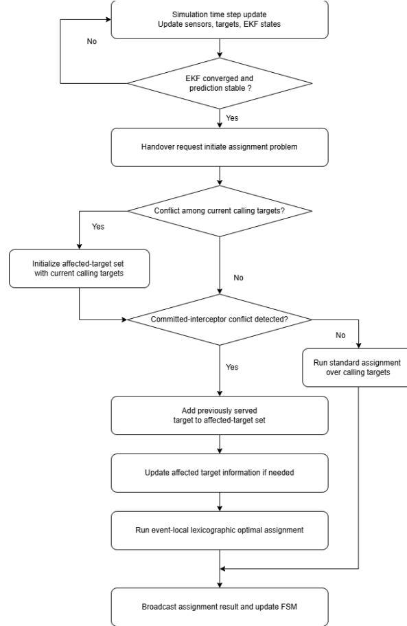
Figure1: Conflict-aware interceptor assignment workflow in the DES framework.
