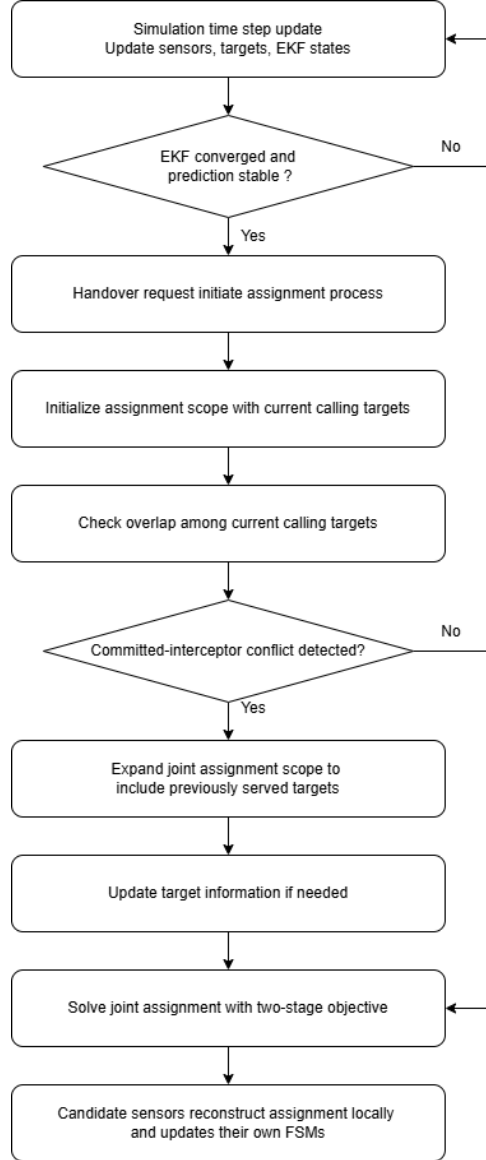
Figure 1: Joint interceptor assignment workflow in the DES framework.
