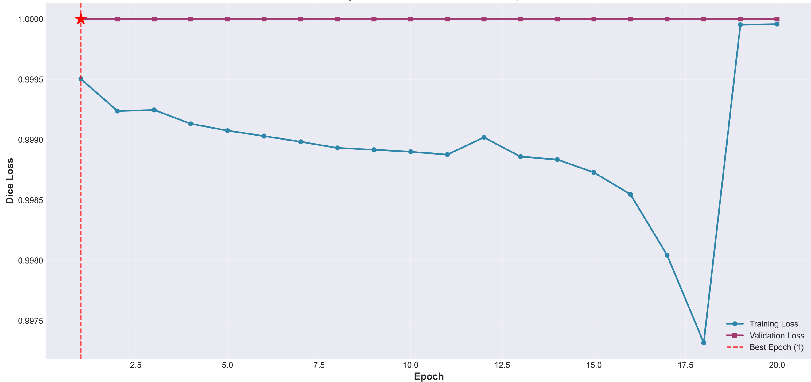
Training and Validation Loss Over Epochs
