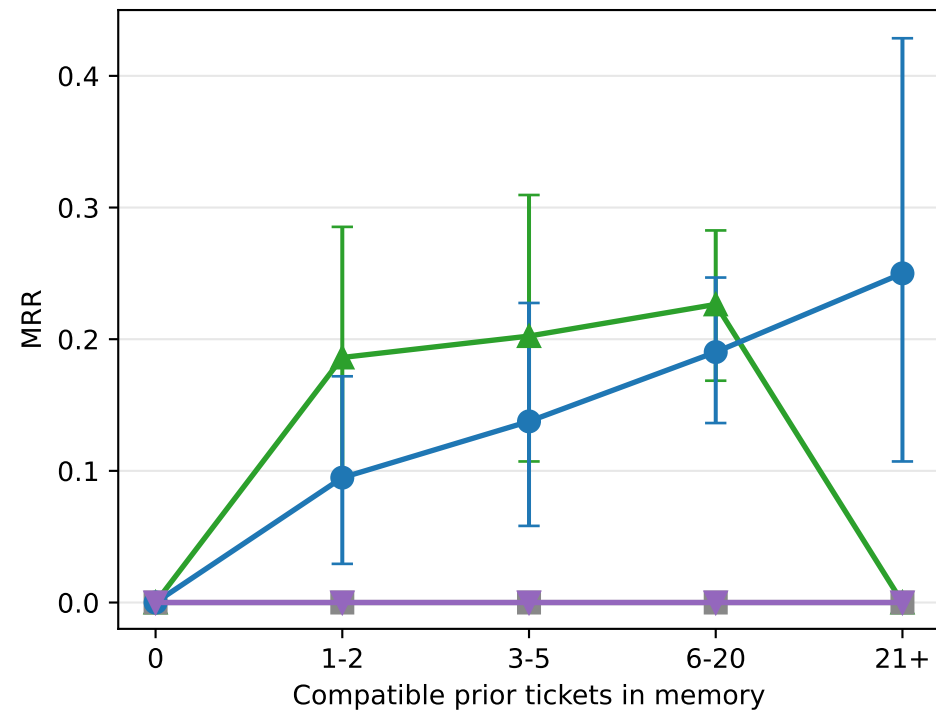
MRR
