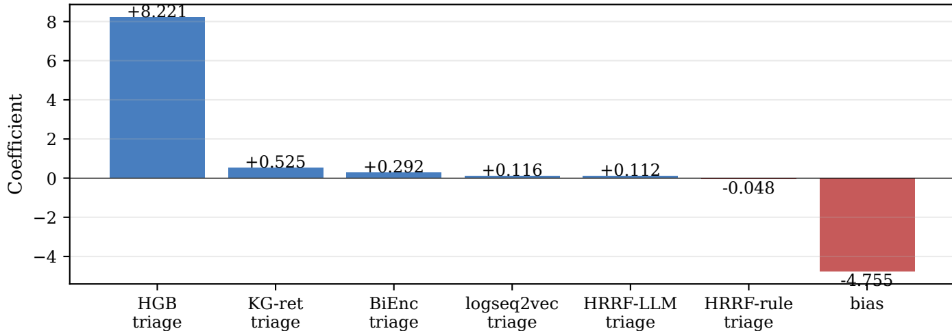
L1 stacker coefficients (LogReg, class-balanced, 5-fold CV)
