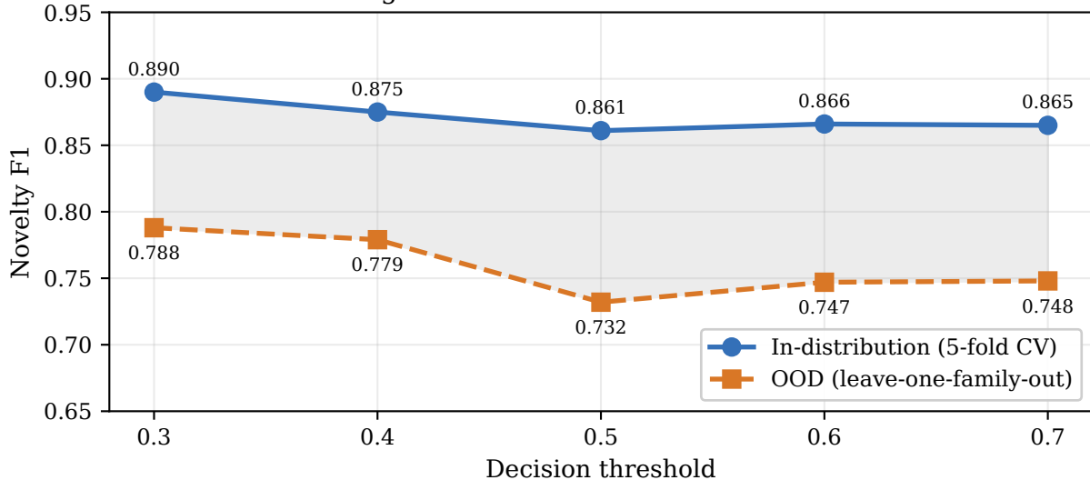
G8: OOD generalization of the G7 learned classifier
