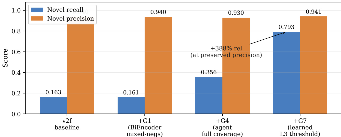
L3 novelty: progression across the G-series KEEP phases
