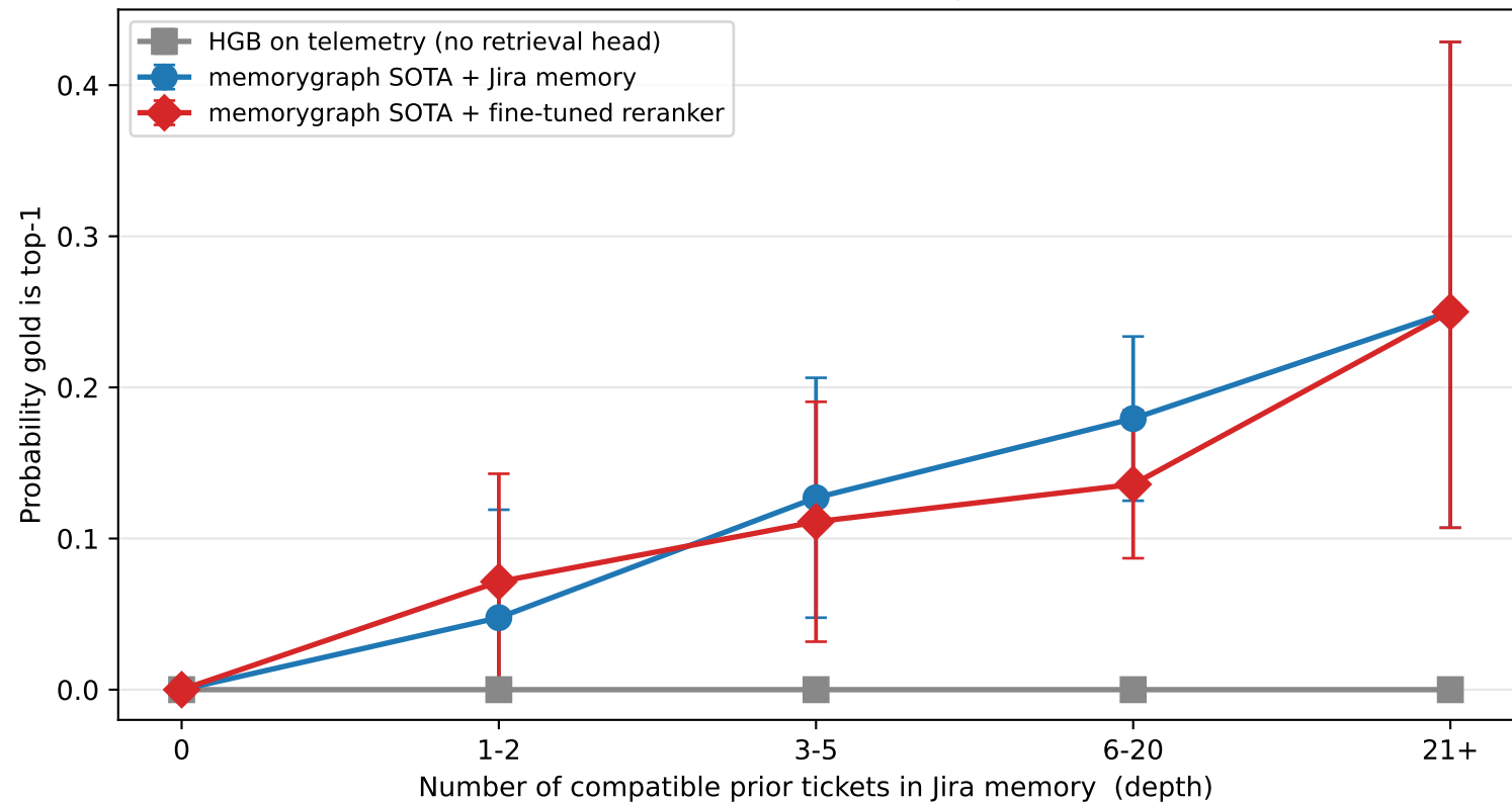
Retrieval quality vs deployment history (Hit@1, 95% bootstrap CI)
