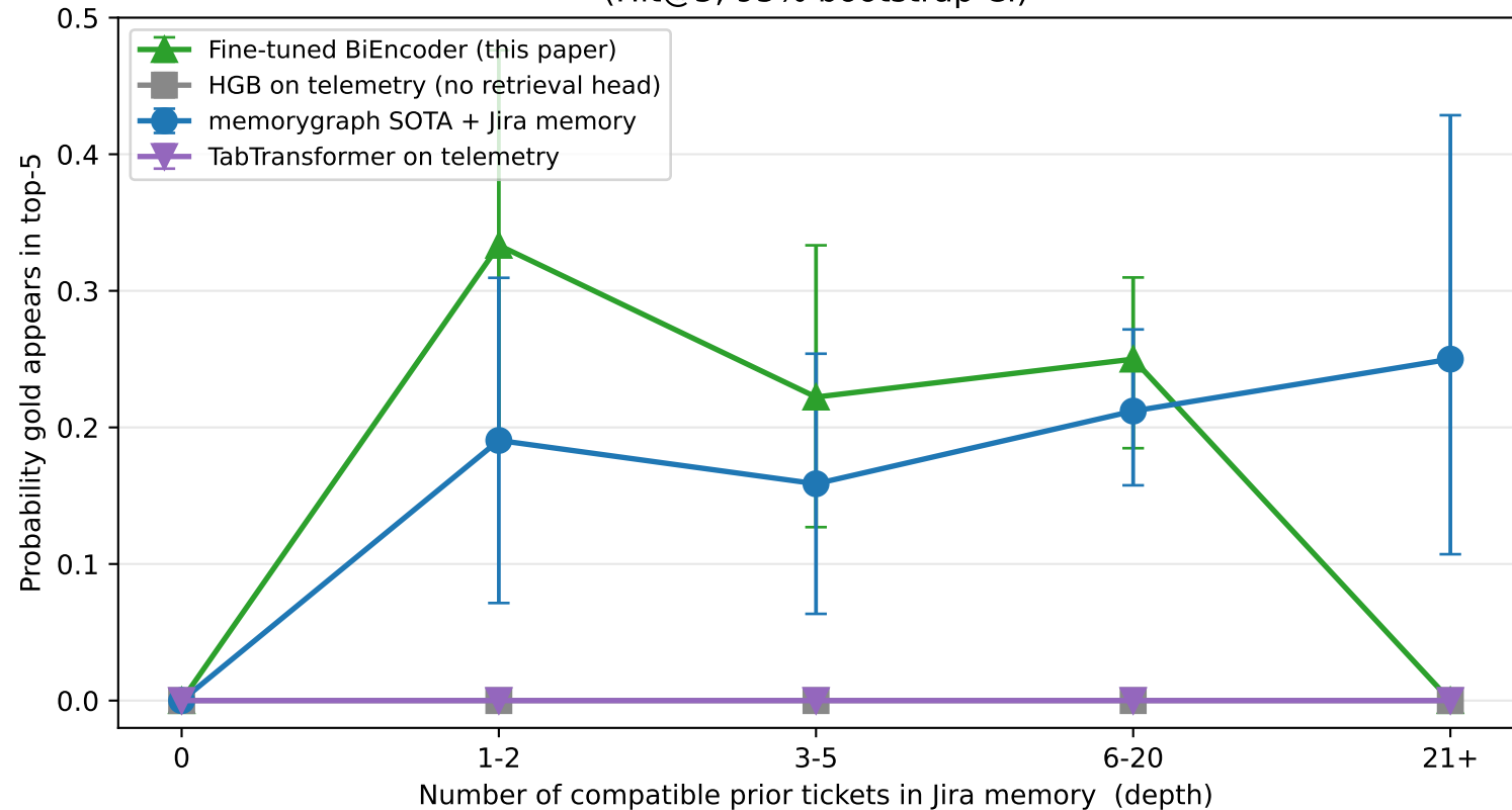
Retrieval quality vs deployment history (Hit@5, 95% bootstrap CI)
