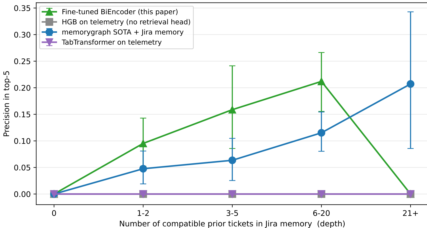
Retrieval quality vs deployment history (Precision@5, 95% bootstrap CI)
